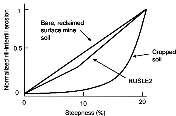
Figure 5.1. Effect of slope steepness on rill-interrill erosion.
